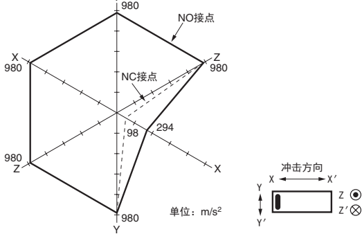
G6RL-1(A)(4)-(ASI)-(PL) 误动作冲击
