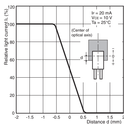
Fig9. Sensing Position Characteristics (Typical)
