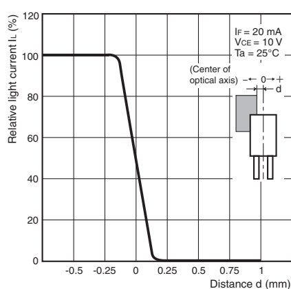
Fig8. Sensing Position Characteristics (Typical)
