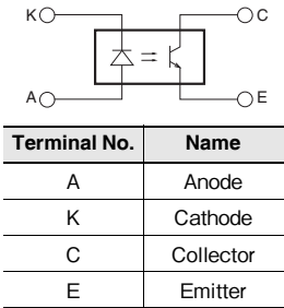
Internal circuit
